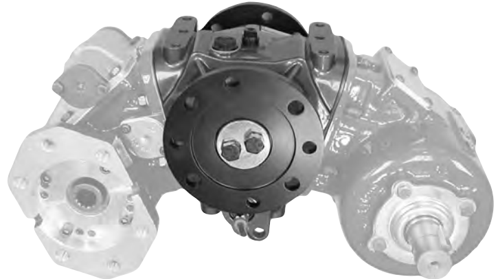
The Muncie Split Shaft PTO Model SS66-U2X3-A00XX (As shown, less PTOs)
