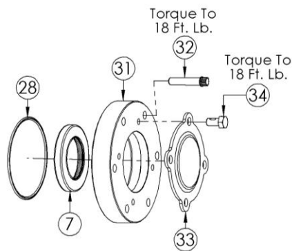
CD10 – Greaseable Bearing Cover Assembly
