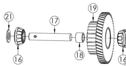
CD10 – Input shaft Assembly
